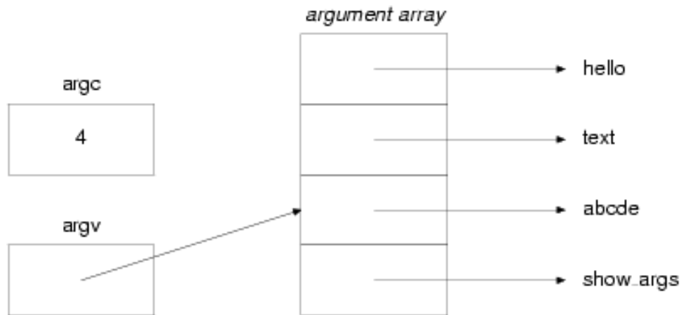
Figure 10.2: Diagram showing the changes to the arrangement in Figure 10.1 after incrementing 'argv' so that it points to the next element in the array of pointers
